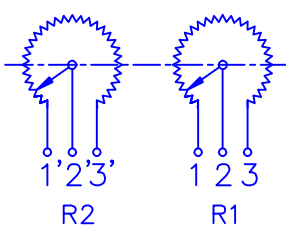
CIRCUIT
